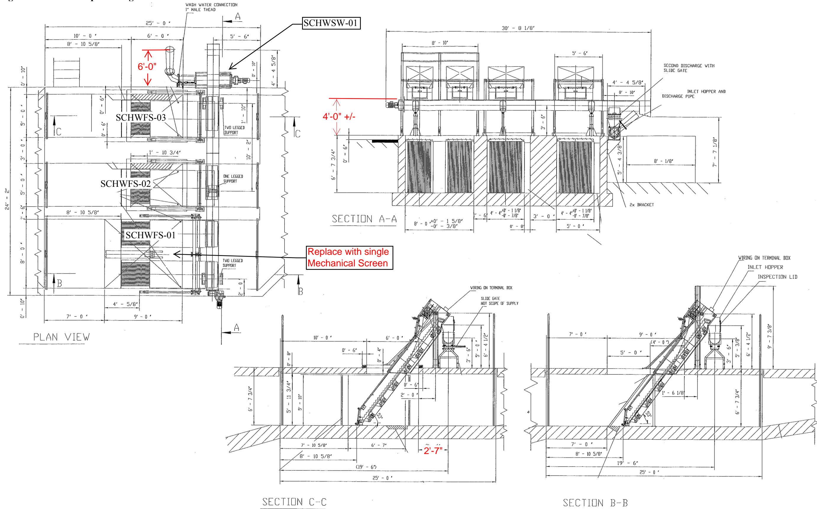
Figure 1- As-Built Shop Drawings
